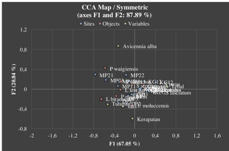
Figure 4. Correspondence analysis output showing correlations between mangrove parameters and the presence of economically important fish species
